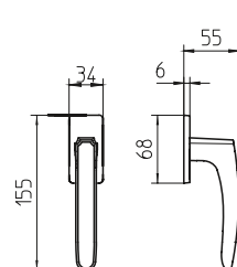
1872/DK martellina dk drehkipp system
