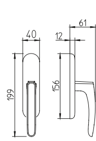
1872/M cremonese window lever handle
