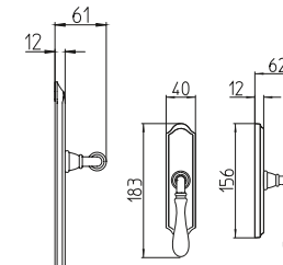
1422/M cremonese window lever handle
