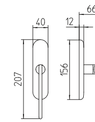
1752/M cremonese window lever handle
