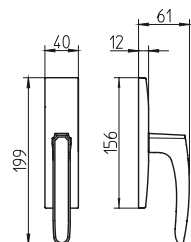
1872/M cremonese window lever handle
