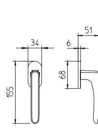
1872/DK martellina dk drehkipp system
