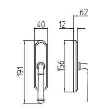
1342/M cremonese window lever handle
